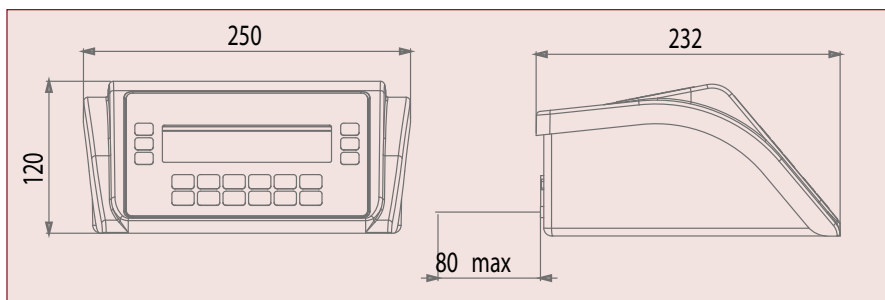
DESK MOUNT VERSION DD700 ABS
