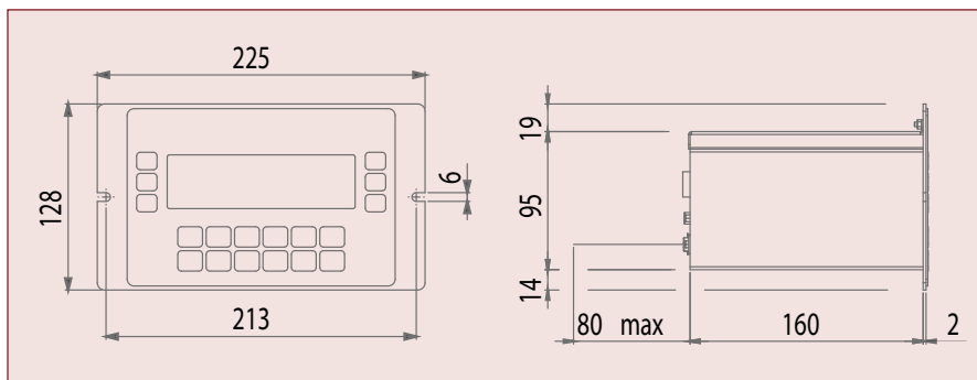
PANEL MOUNT VERSION
